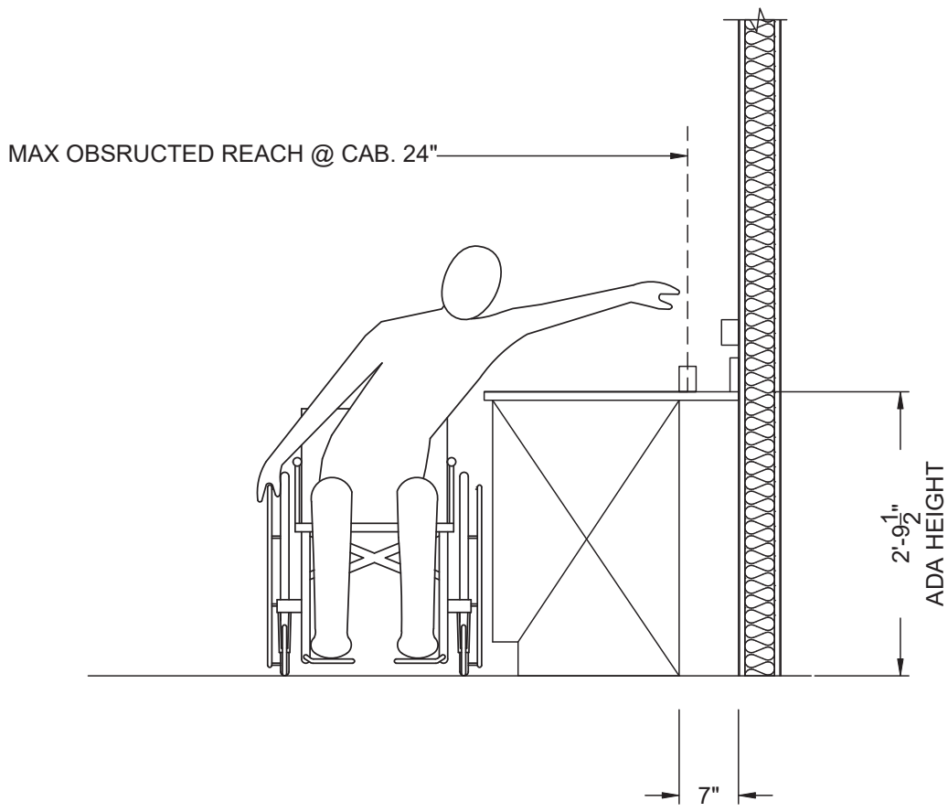
TYP. ADA OBSTRUCTED REACH @ CASEWORK SCALE: 3/4" = 1'-0"
